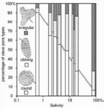
Sieve pores in Cyprideis torosa
