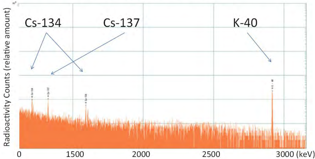
\gamma -Ray Spectrum of rice grains
