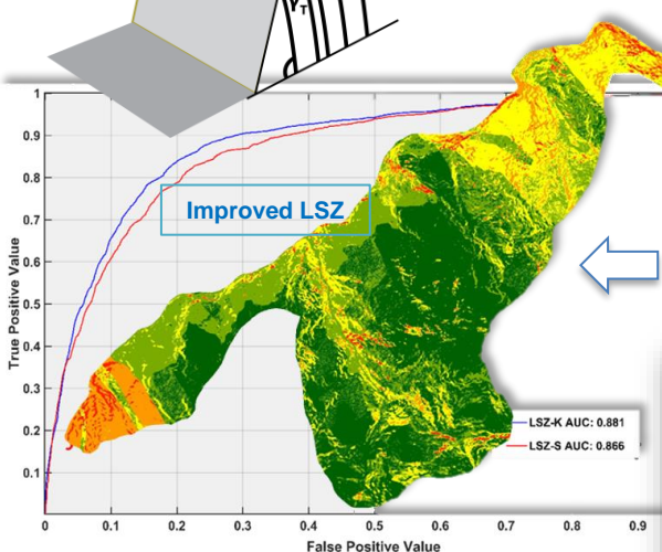
Landslide susceptibility zonation (LSZ)
