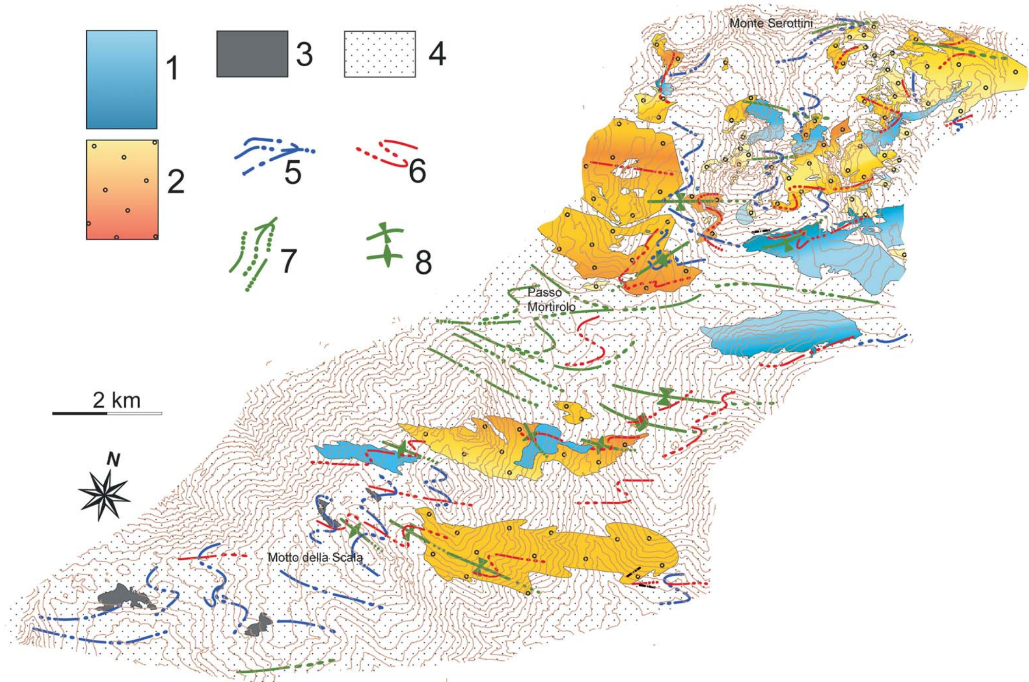
Fig. 6*- Simplified geological map of km-scale strain gradients and related structures within Permian-age metaintrusives. Legend: Colour gradients identify fabric gradients, from coronitic to mylonitic fabrics, within metadiorites (1) and metagranitoids (2); 3) Grt-bearing pegmatites; 4) undifferentiated country rocks of Permian intrusives; foliation trajectories are shown for S1 and S2 foliations (5), S3 (6), S4 and S5 (7); axial plane trajectories are also reported (8).
