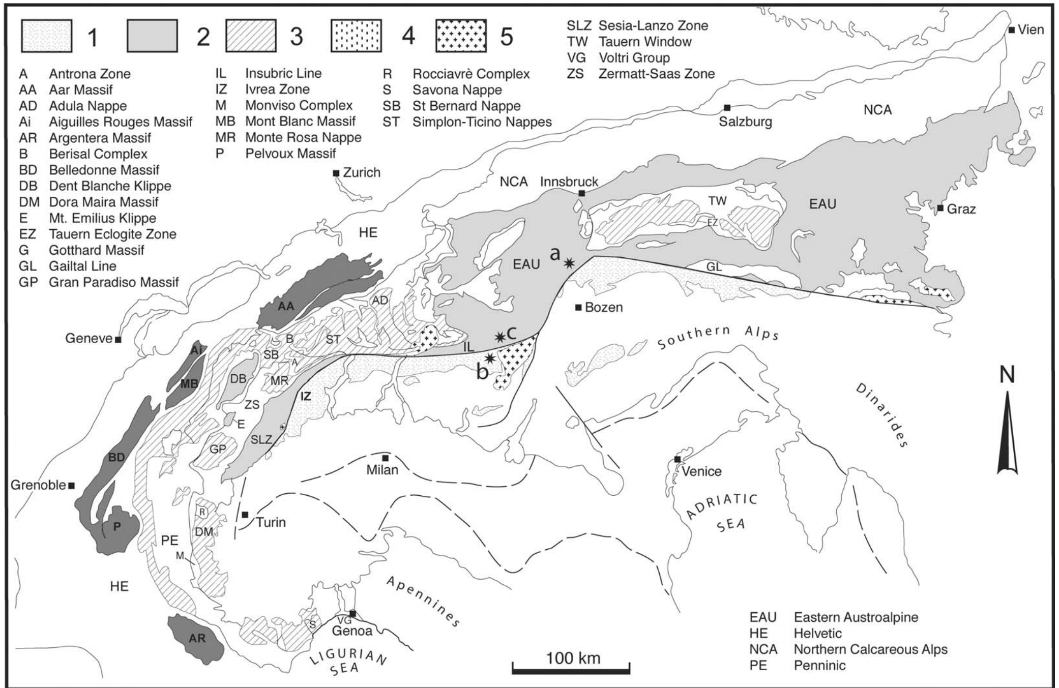
Fig. 1* –Tectonic sketch map of the Alpine chain: shaded areas correspond to continental Alpine crust. Legend: 1 = Southalpine basement; 2 = Austroalpine basement; 3 = Penninic basement; 4 = Helvetic basement; 5=Tertiary intrusive stocks. Stars localise the Texel Gruppe metapelites in the Oetztal nappe (a), the Eastern Orobic Alps metapelites in the Central Southern Alps (b) and the Mortirolo Pass area in Central Austroalpine domain of the Languard-Campo Nappe (c).
